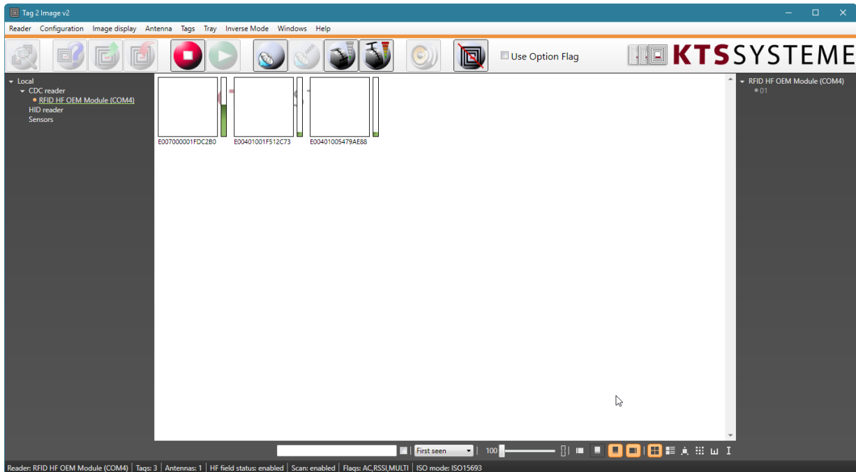
Figure 6: KTS Tag2Image
